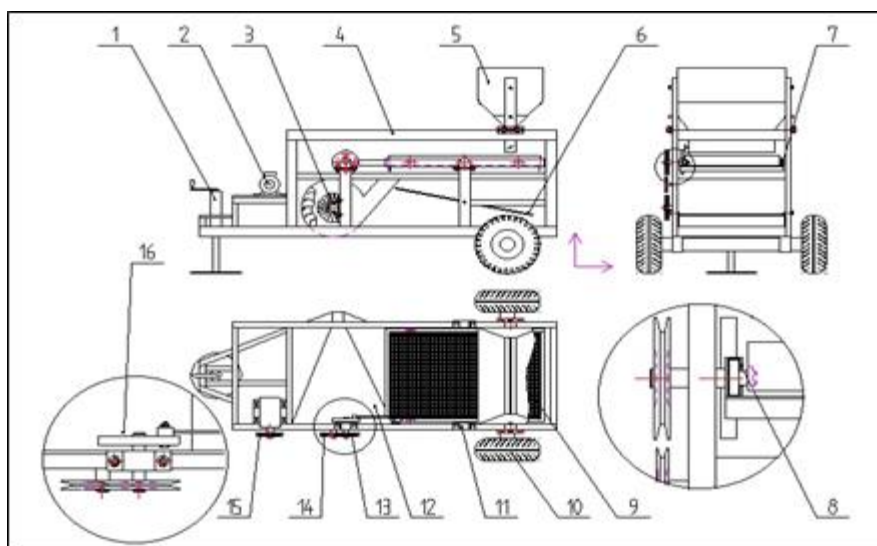
Figure 1: The major components of the prototype of wheat cleaner
