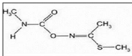
Fig 1: Chemical structure of Methomyl
